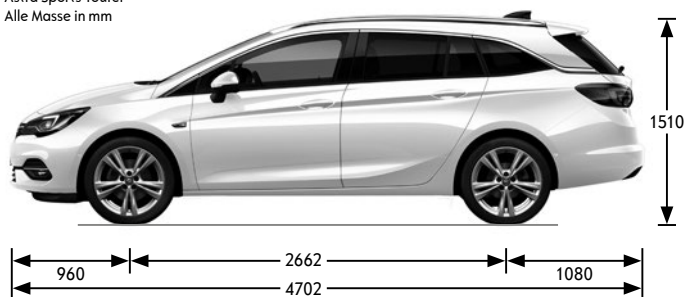
Astra Sports Tourer Alle Masse in mm
